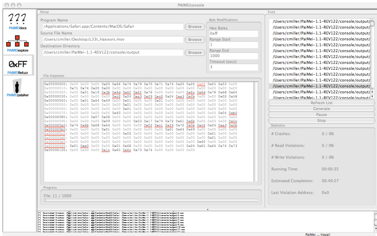
Figure 1: PAIMEI fuzz for Mac OS X in action
