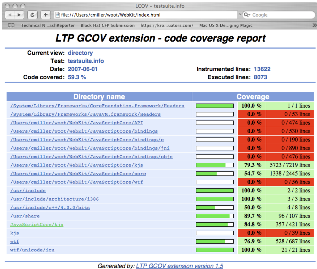
Figure 5: LCOV generated code coverage information for WebKit.
