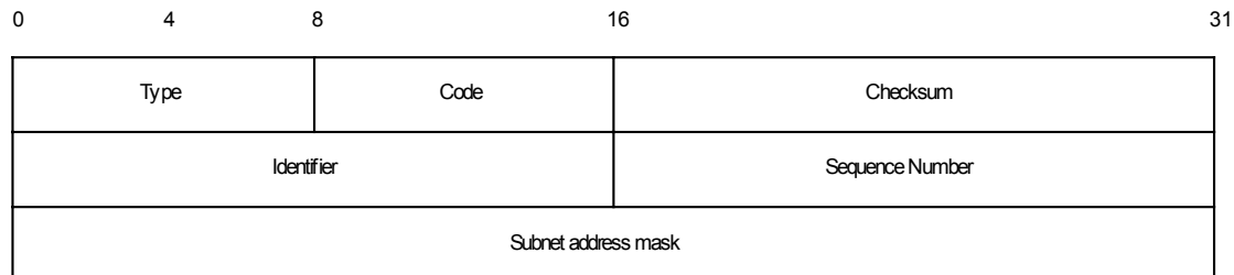
Figure 5: ICMP Address Mask Request & Reply message format
