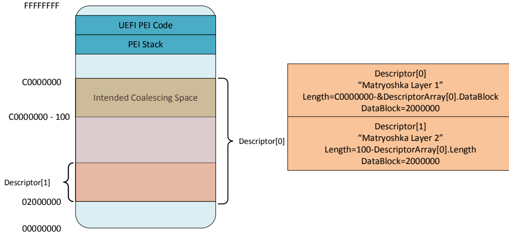
Figure 12: The Matryoshka descriptor configuration. Sum of length values overflows 32 bit Integer.
