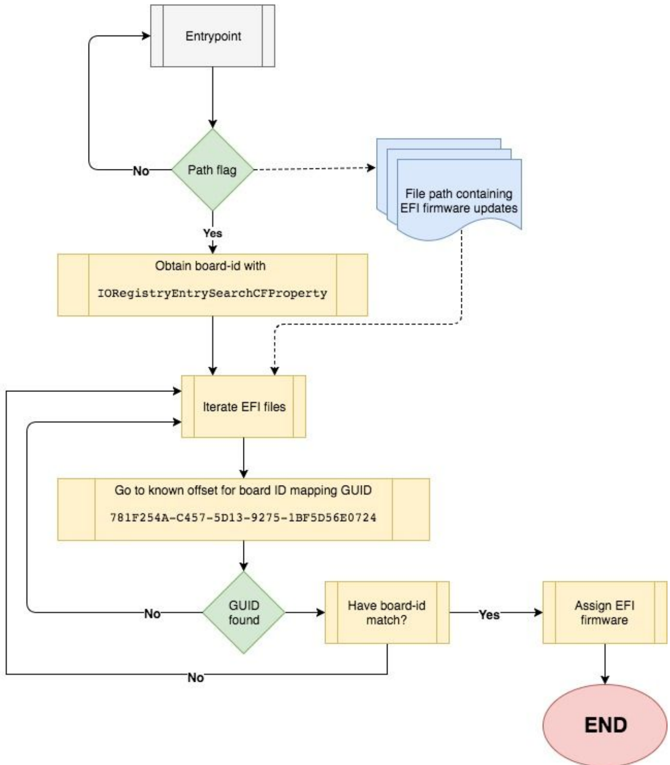
Figure 3 - Flow diagram of the process efiupdater follows to locate the correct EFI update file
