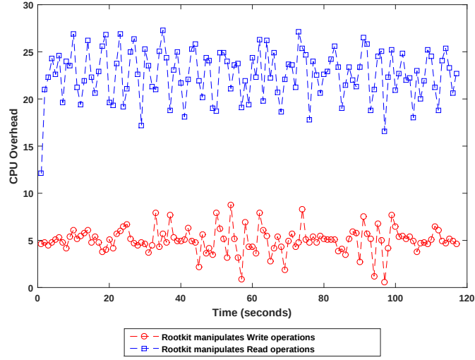
Fig. 10. CPU overhead in rootkit based Pin Control attack
