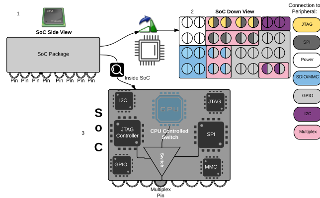
Fig. 3. Part 1 shows an SoC from the Side view. Part 2 shows the design of multiple multiplex pins with different I/O peripheral. Part 3 shows how SoCs peripherals are located inside a SoC and how one multiplex pin is connected to two peripheral.
